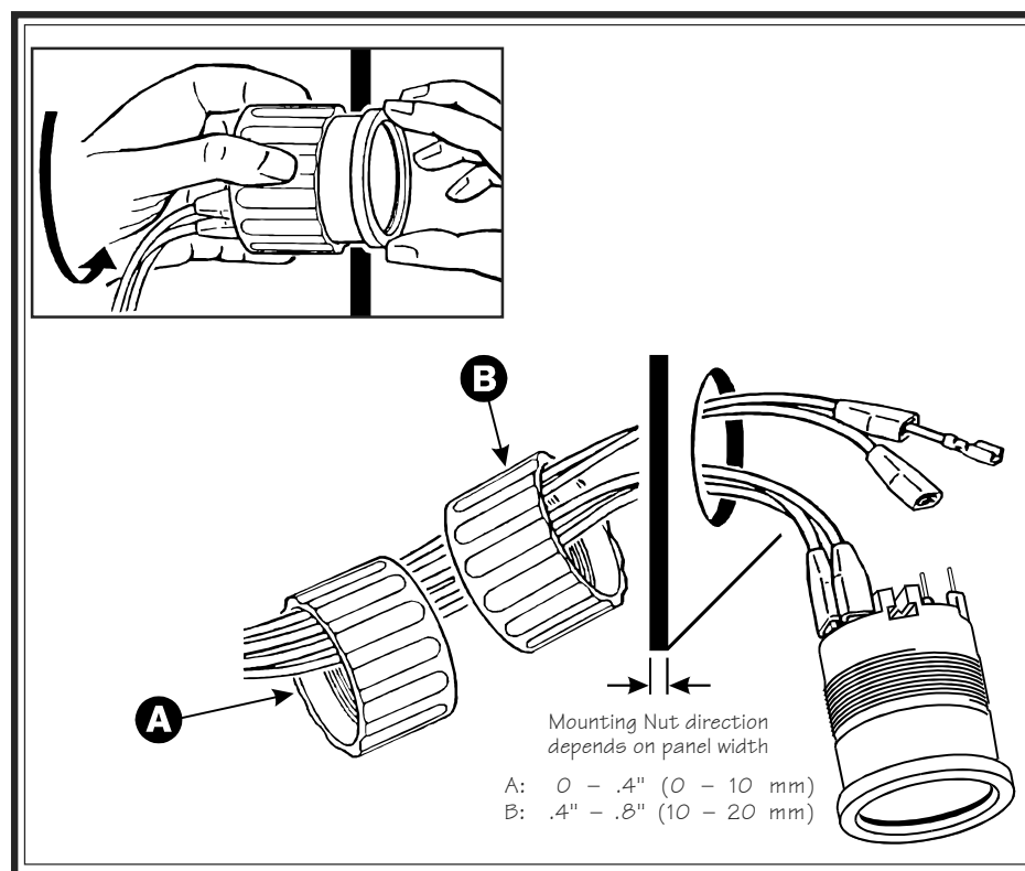
Diagram B Proper mounting using VDO's Spin-Lok™ Mounting Clamp
